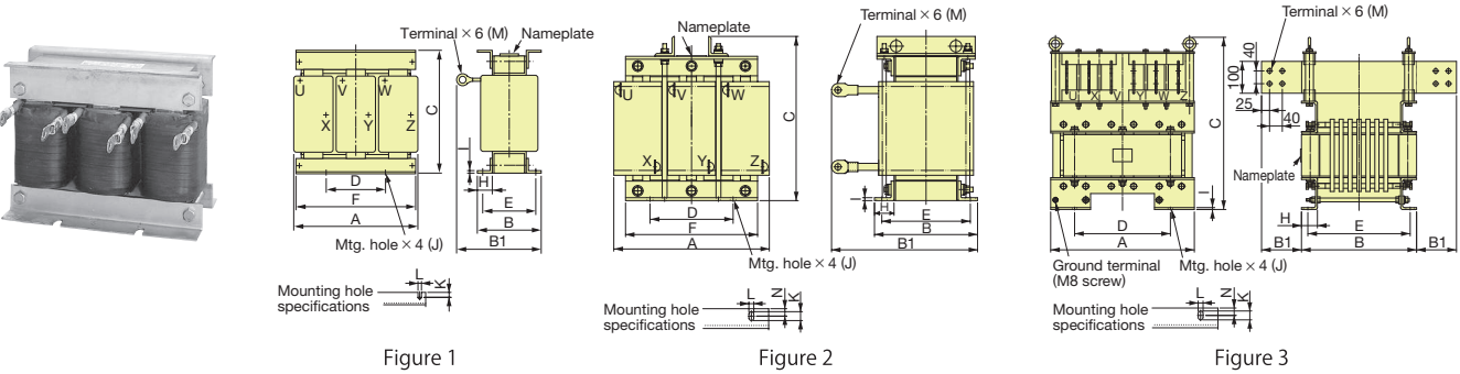
Input AC Reactor 1 200 V Class
